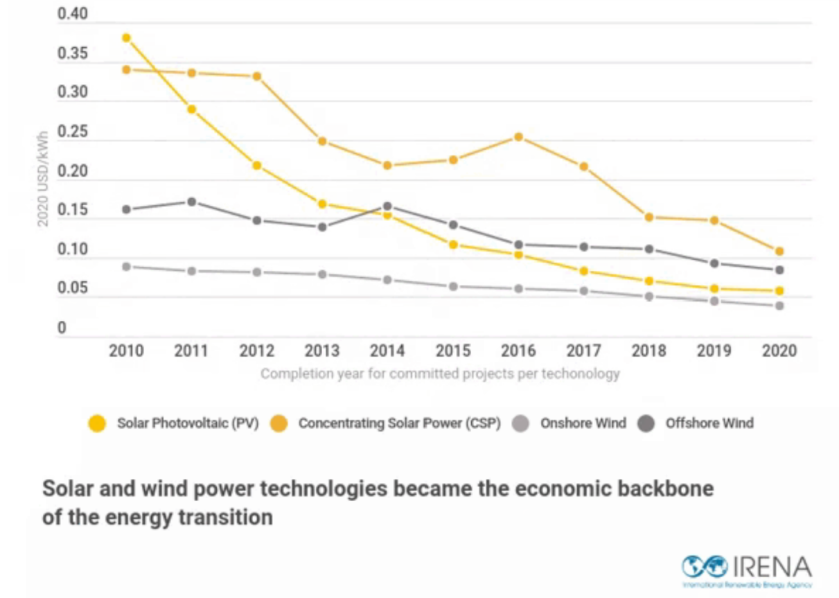
Figure 6 The unit price (USD/kWh) of renewable energies from 2010 to 2020.
