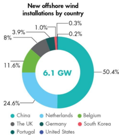
Figure 5 The percentage of new offshore wind installations by country in 2020.
